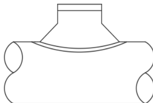
CONICAL SADDLE
